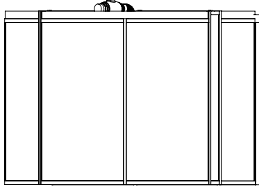
REAR ELEVATION
